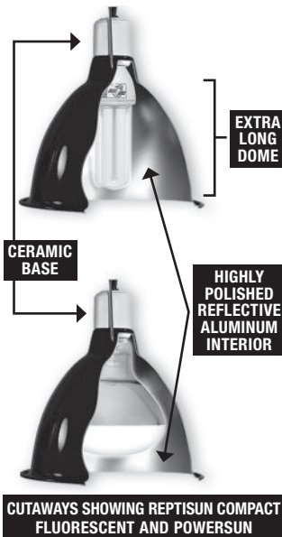
DEEP DOME LAMP FIXTURE SUSPENDED FROM REPTILE LAMP STAND
